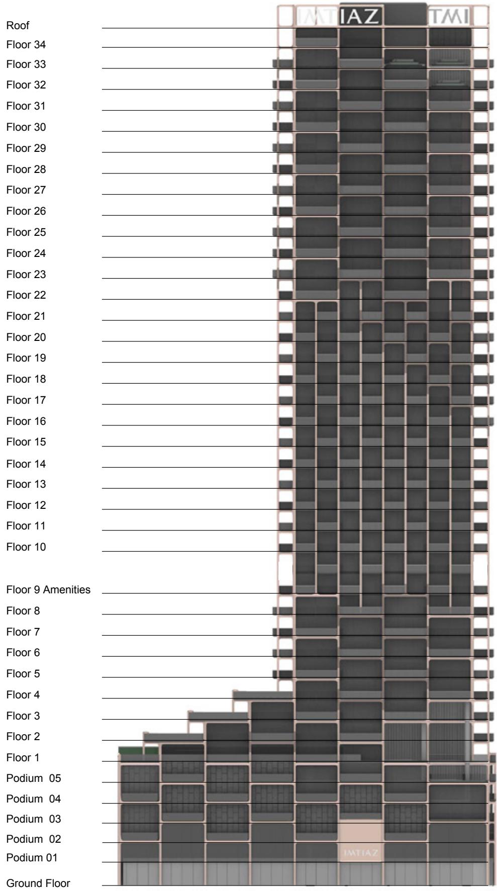
North Elevation
