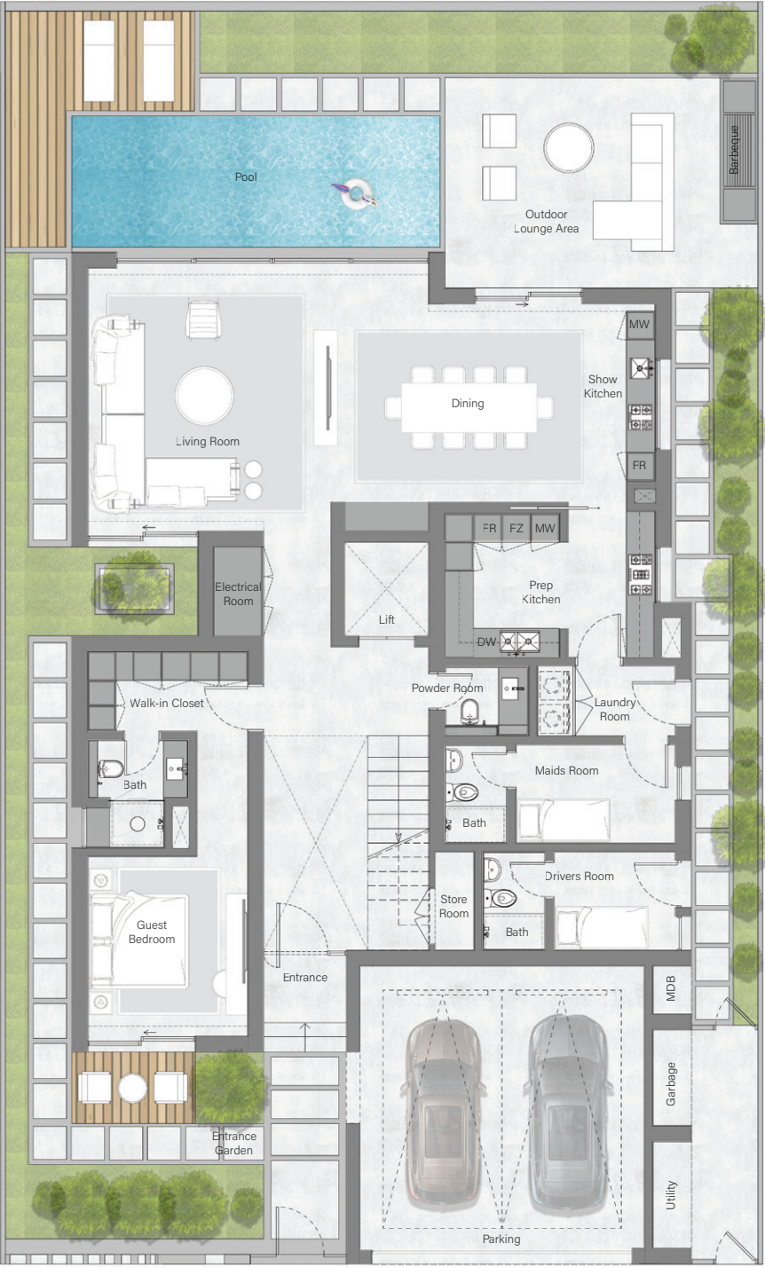
Ground Floor
