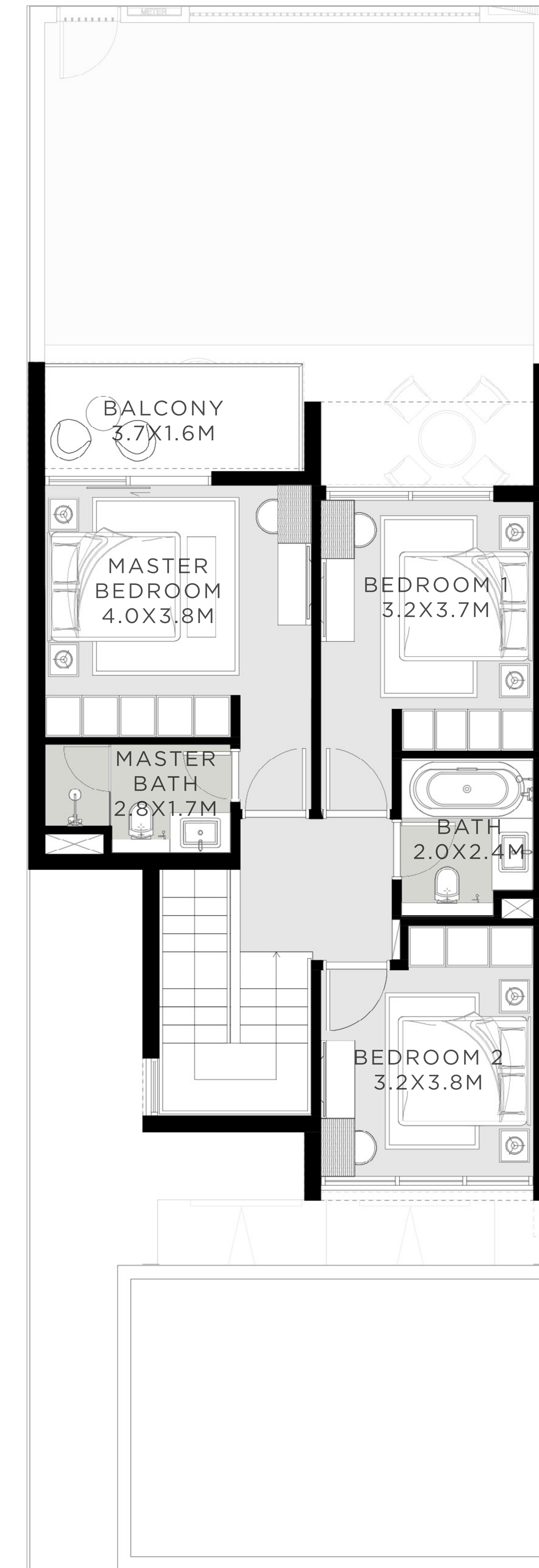
FIRST FLOOR
