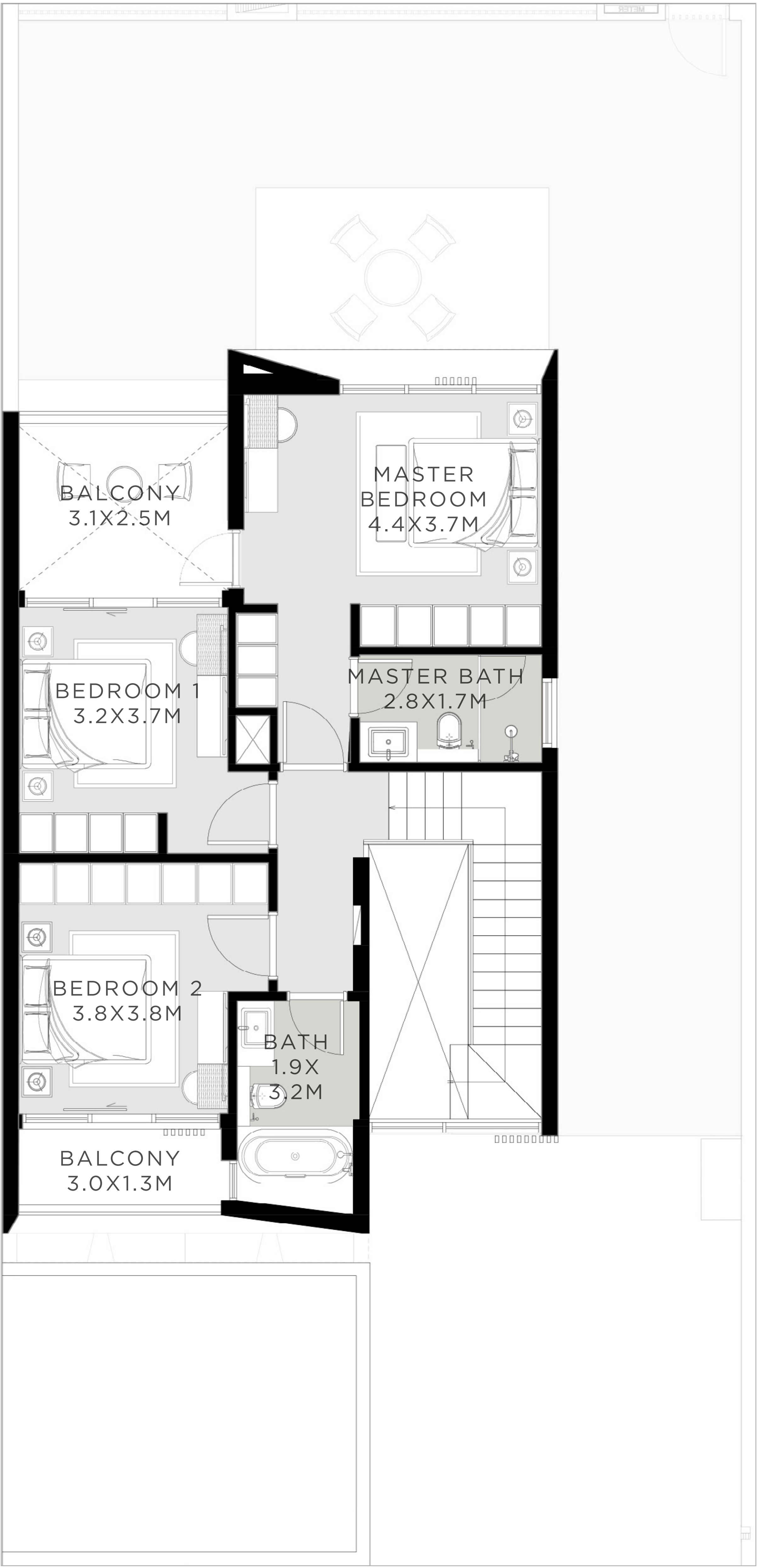
FIRST FLOOR
