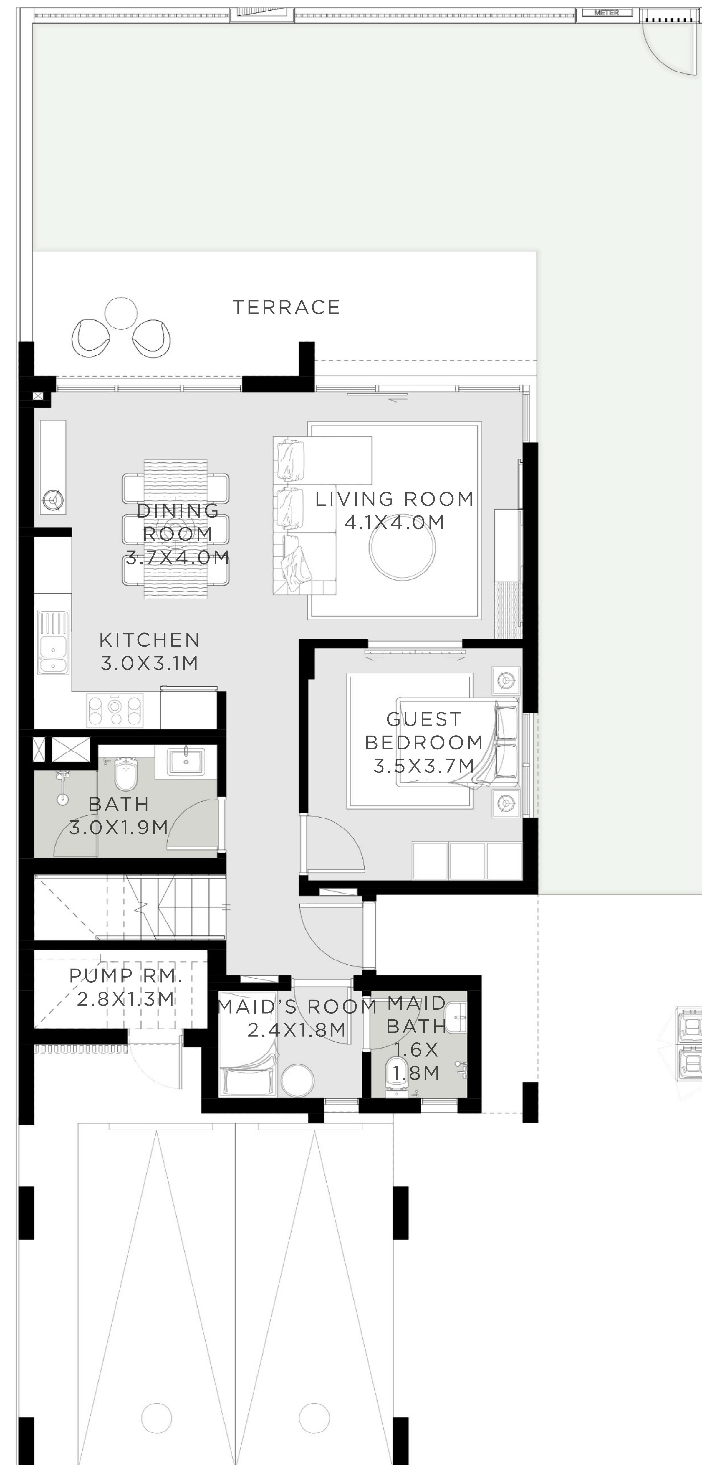
GROUND FLOOR
