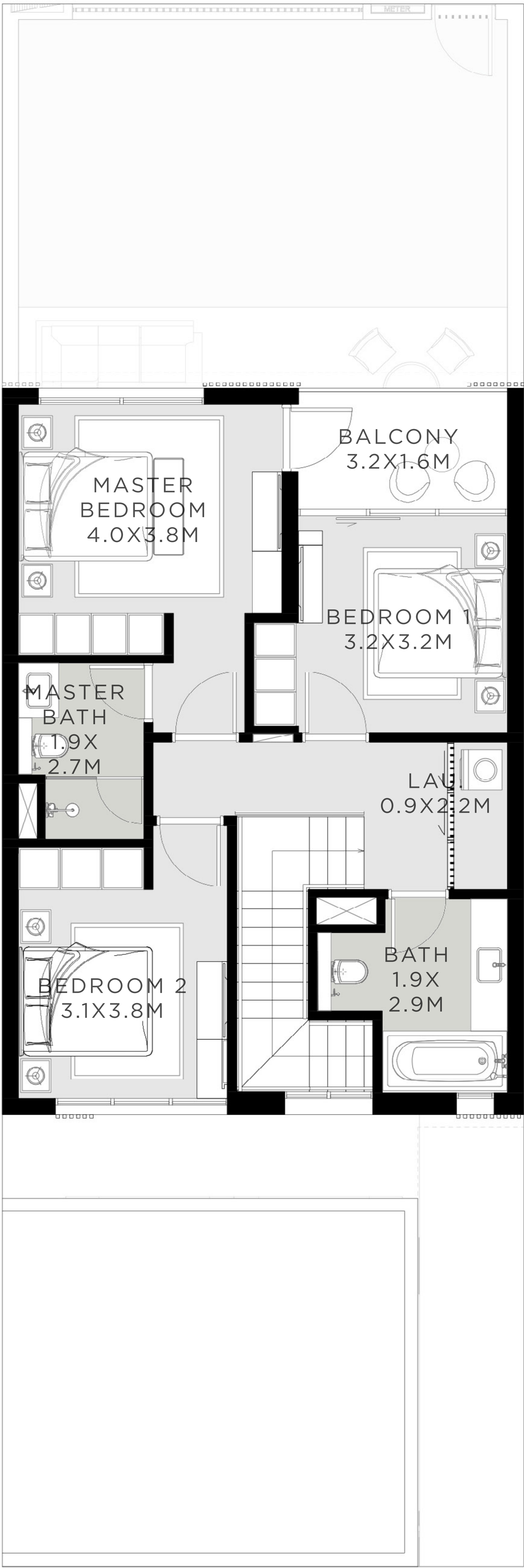
FIRST FLOOR
