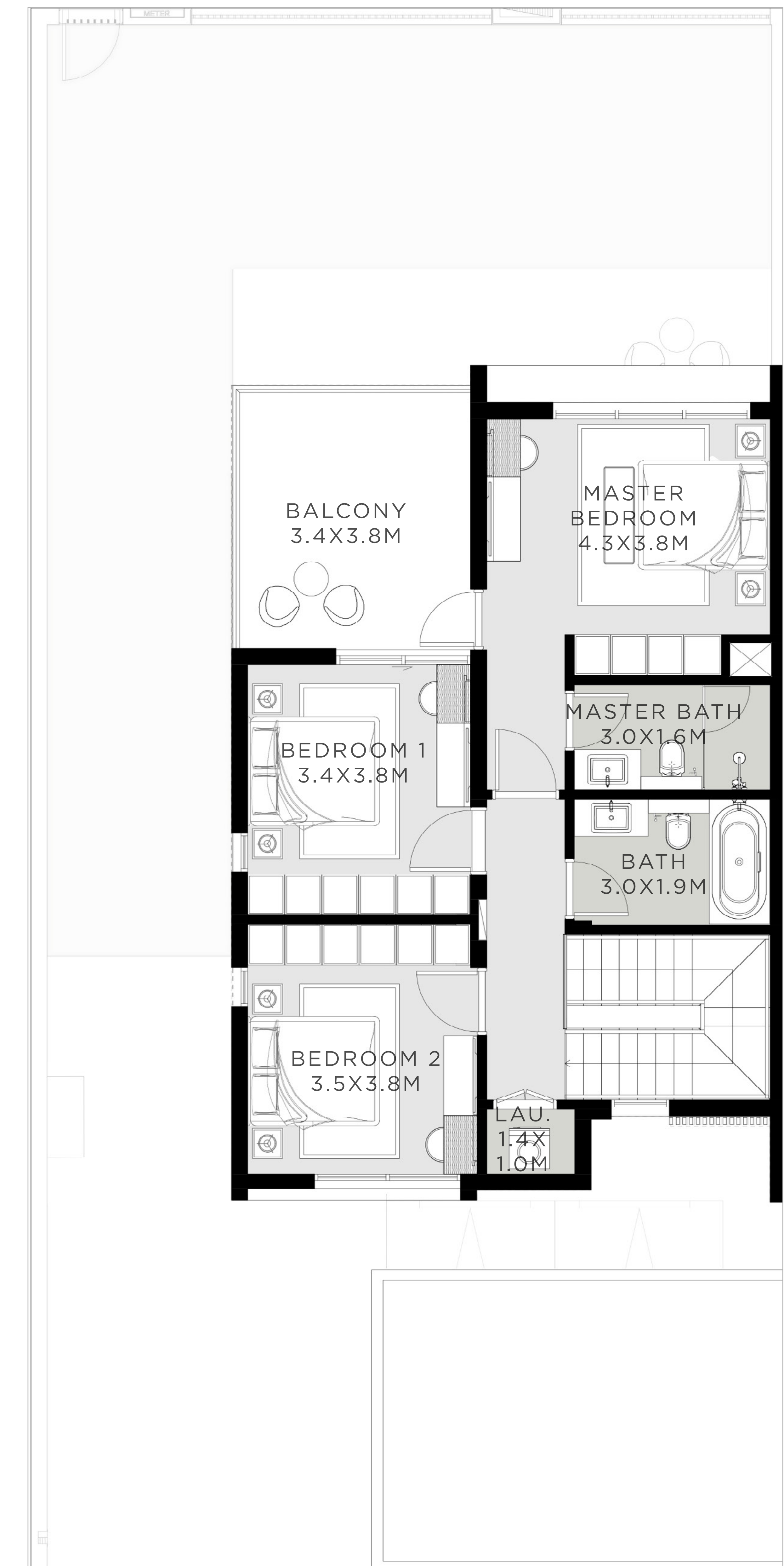
FIRST FLOOR
