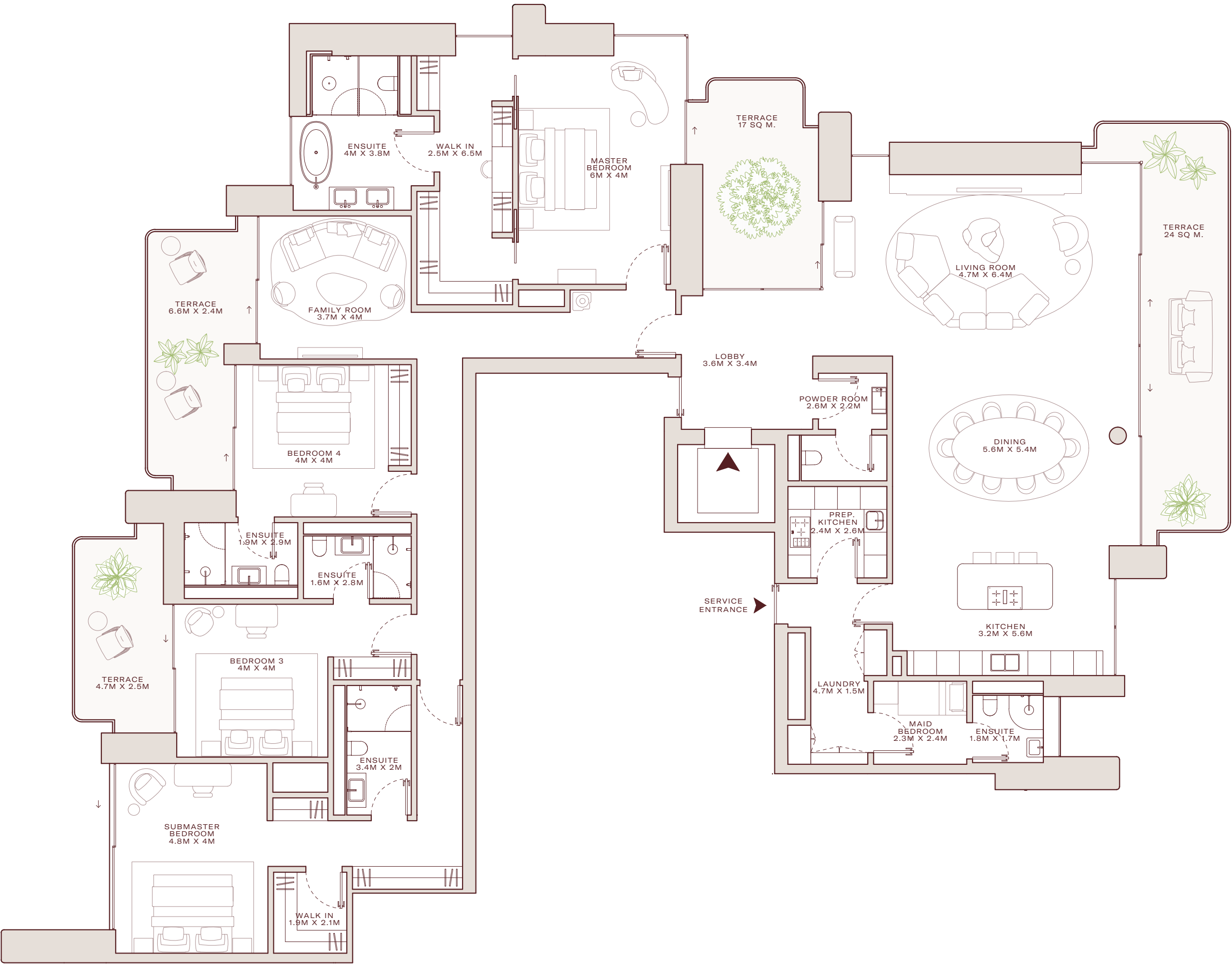
BUILDING FLOORPLATE
