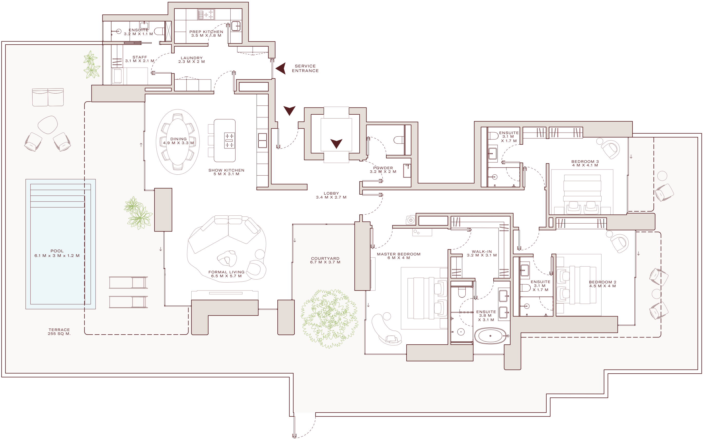
BUILDING FLOORPLATE
