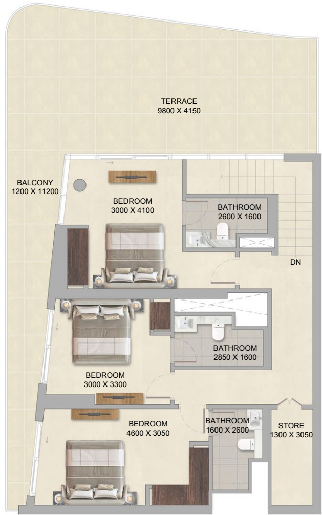
UPPER LEVEL
