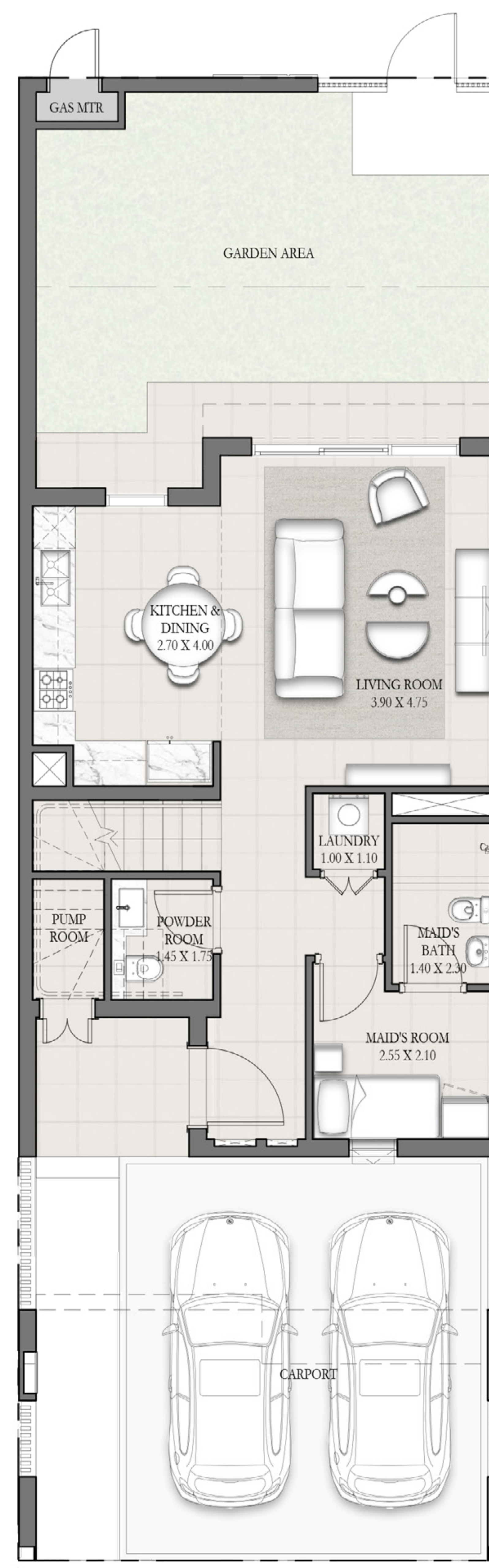
GROUND FLOOR
