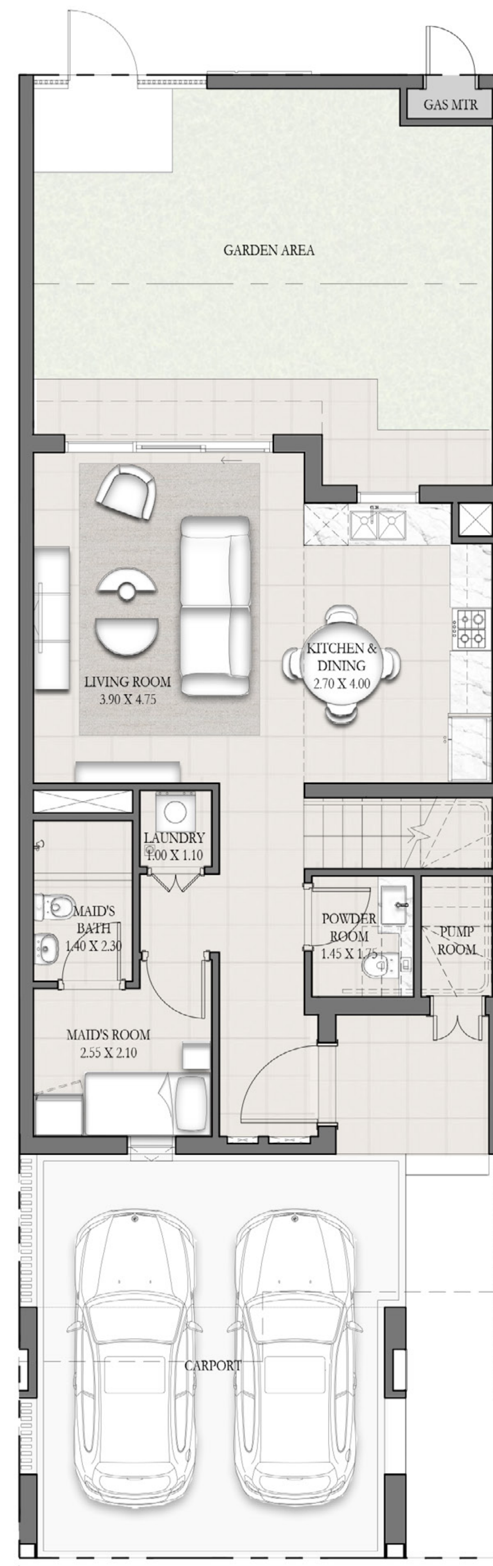
GROUND FLOOR
