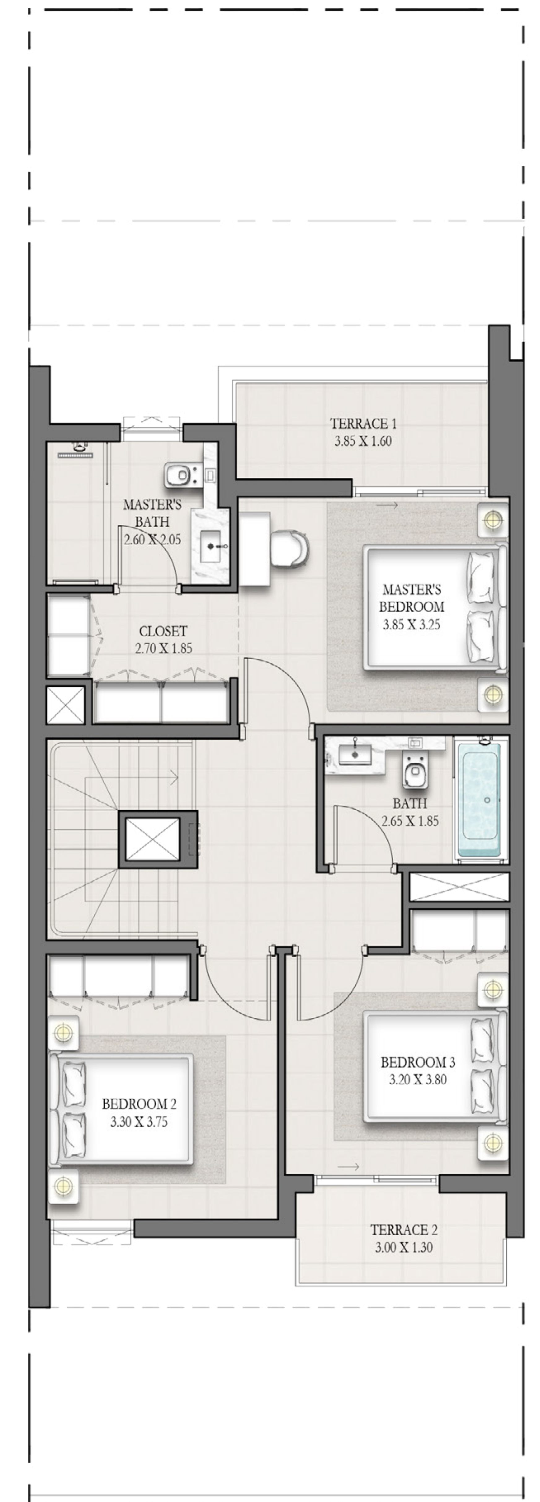
FIRST FLOOR
