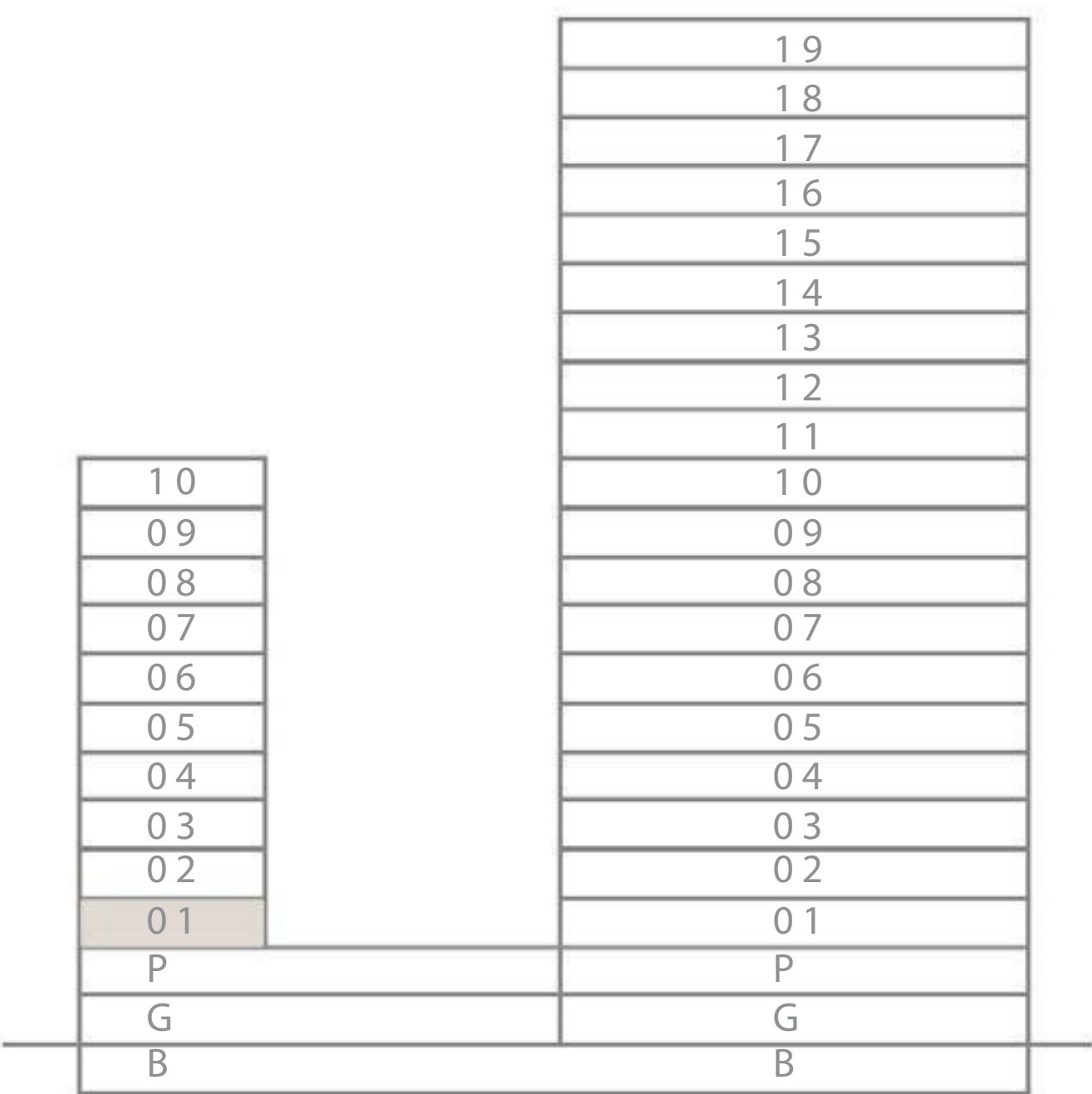
SECTION
