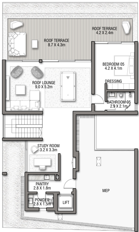
SECOND FLOOR
