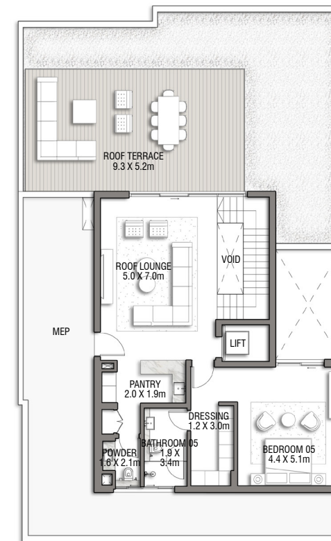
SECOND FLOOR
