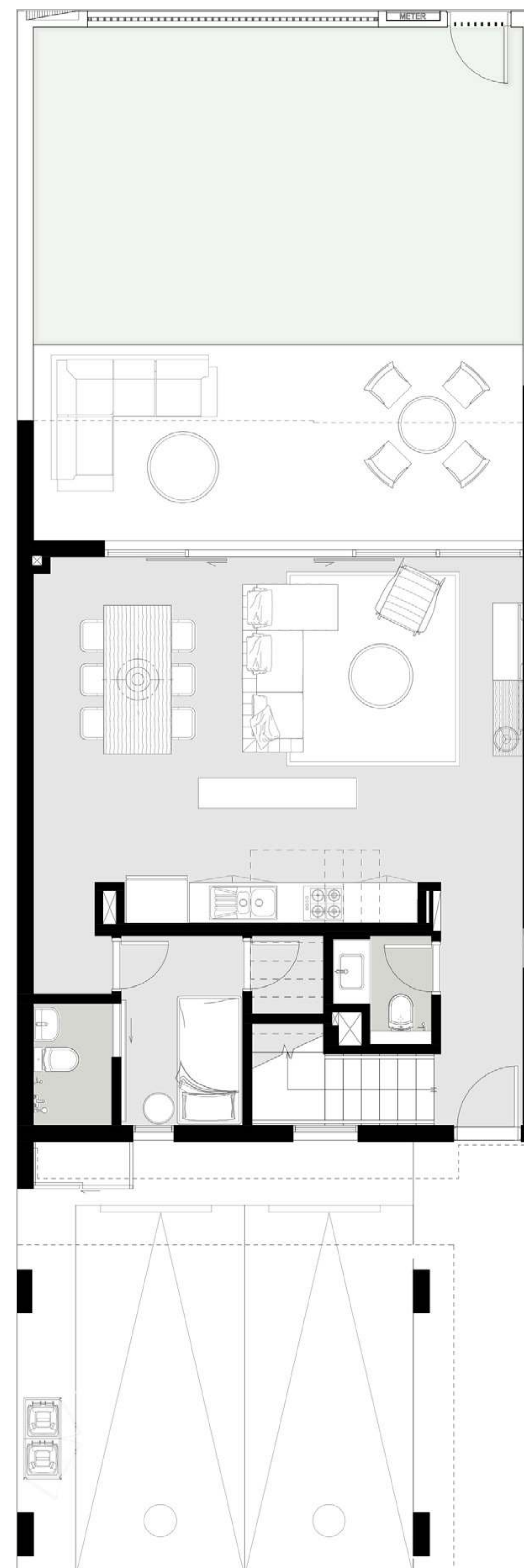
GROUND FLOOR
