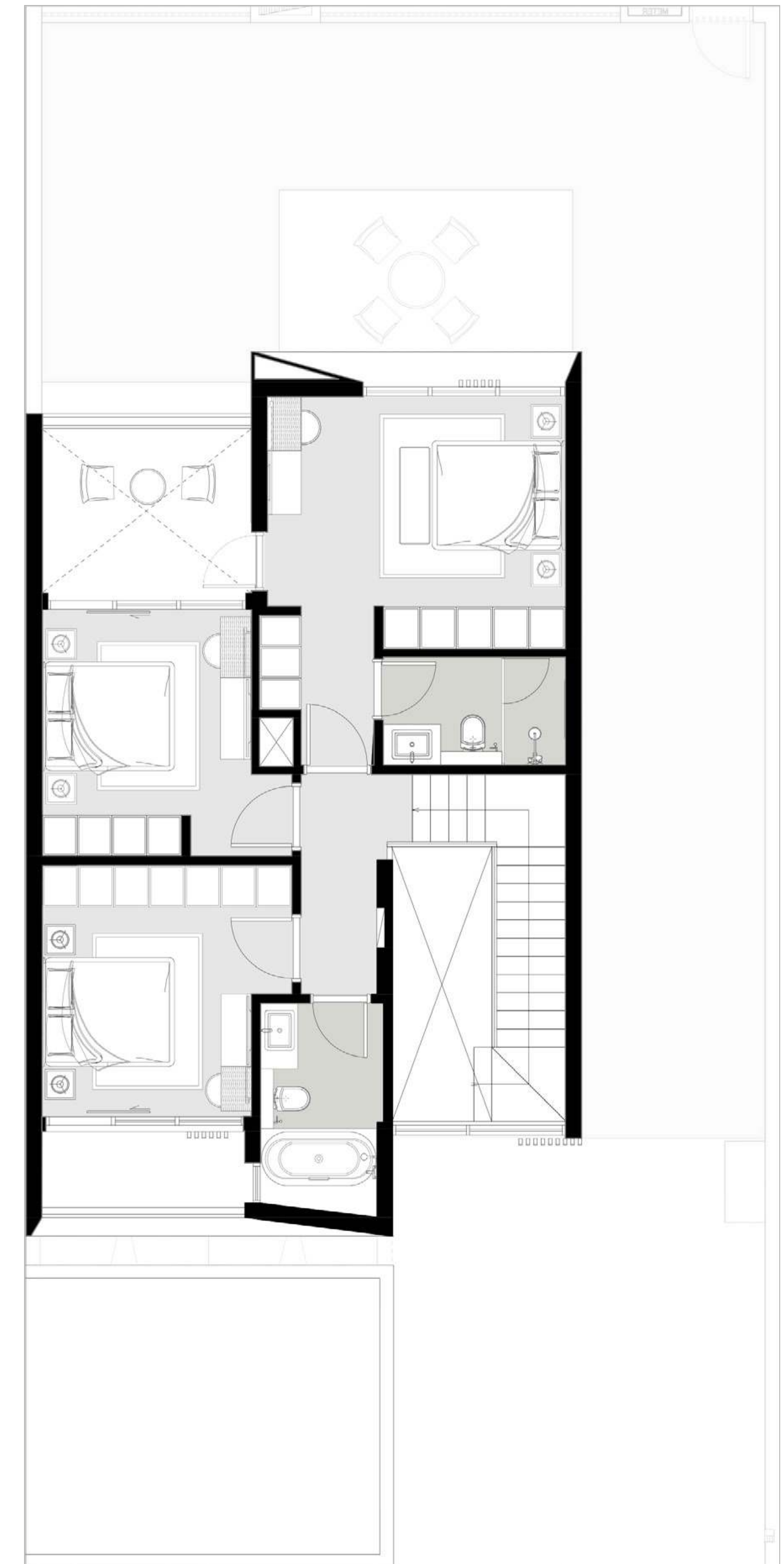
FIRST FLOOR
