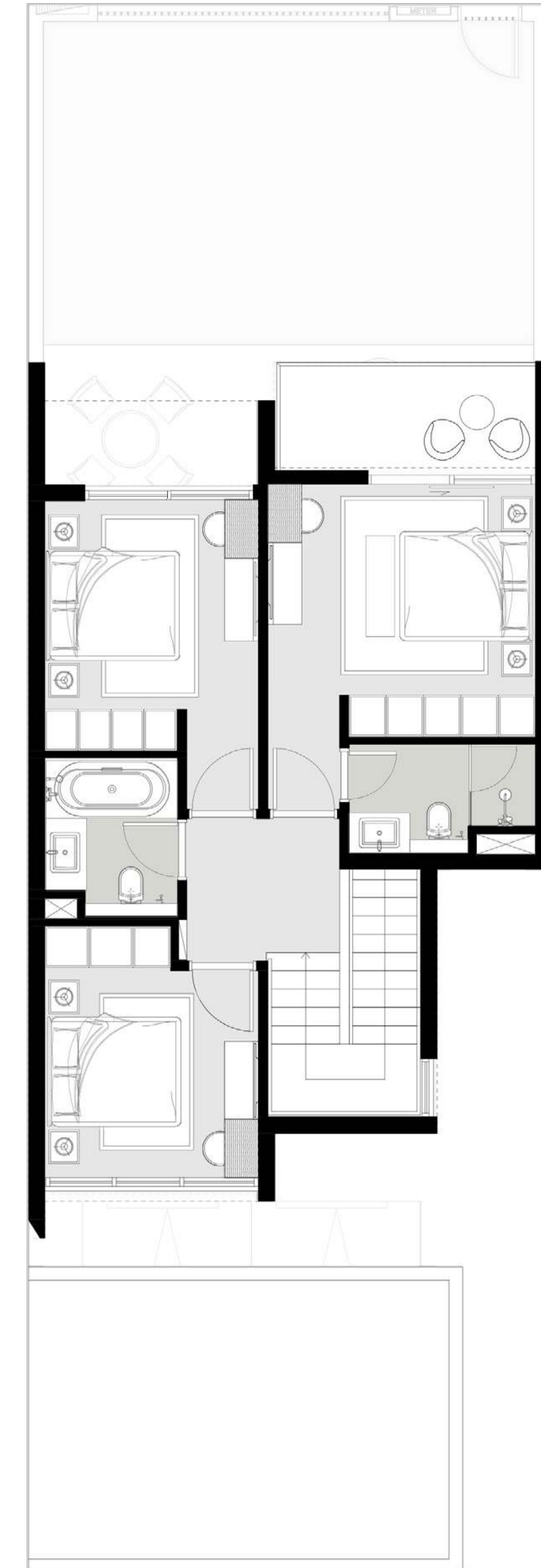
FIRST FLOOR
