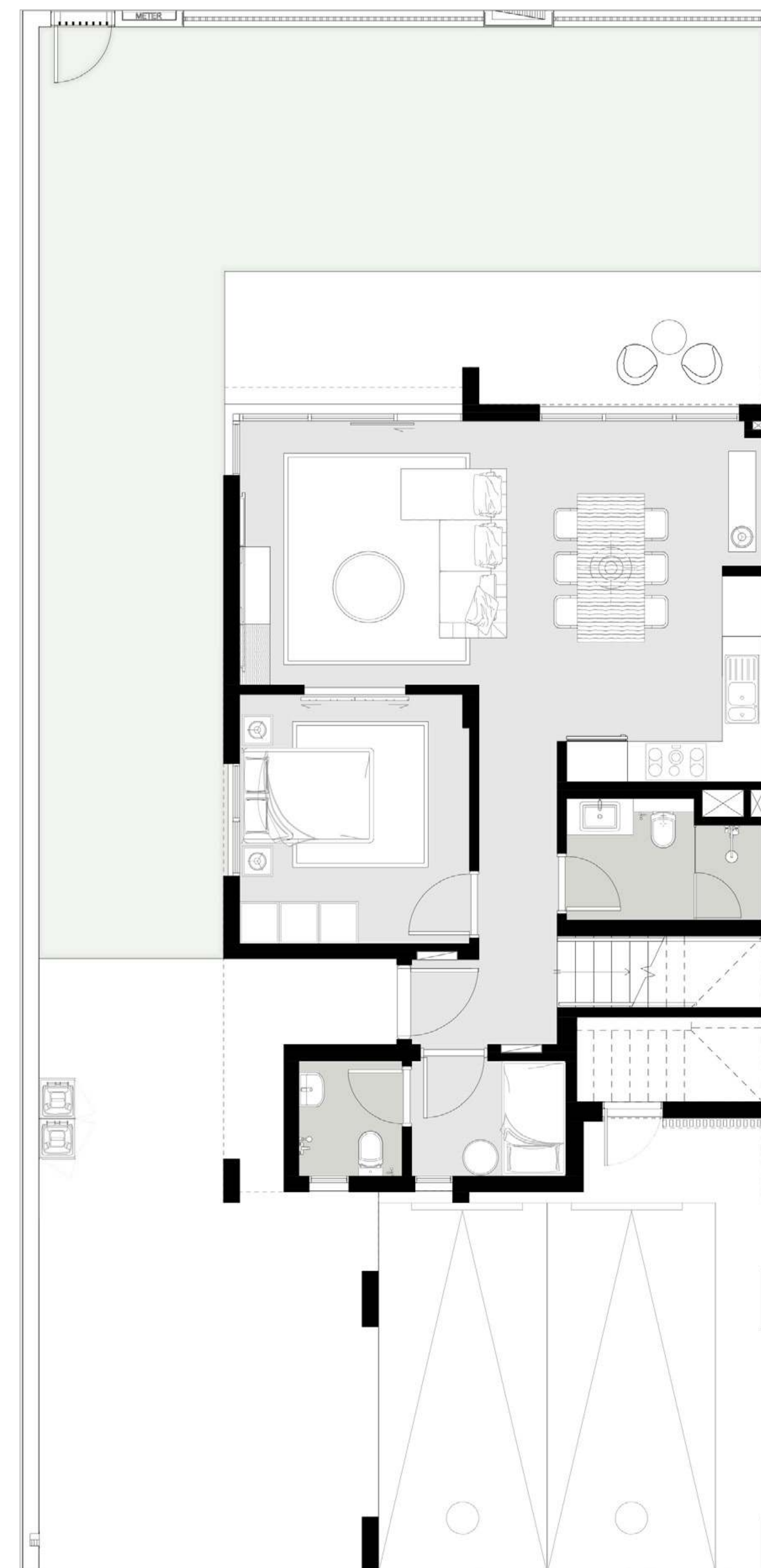
GROUND FLOOR
