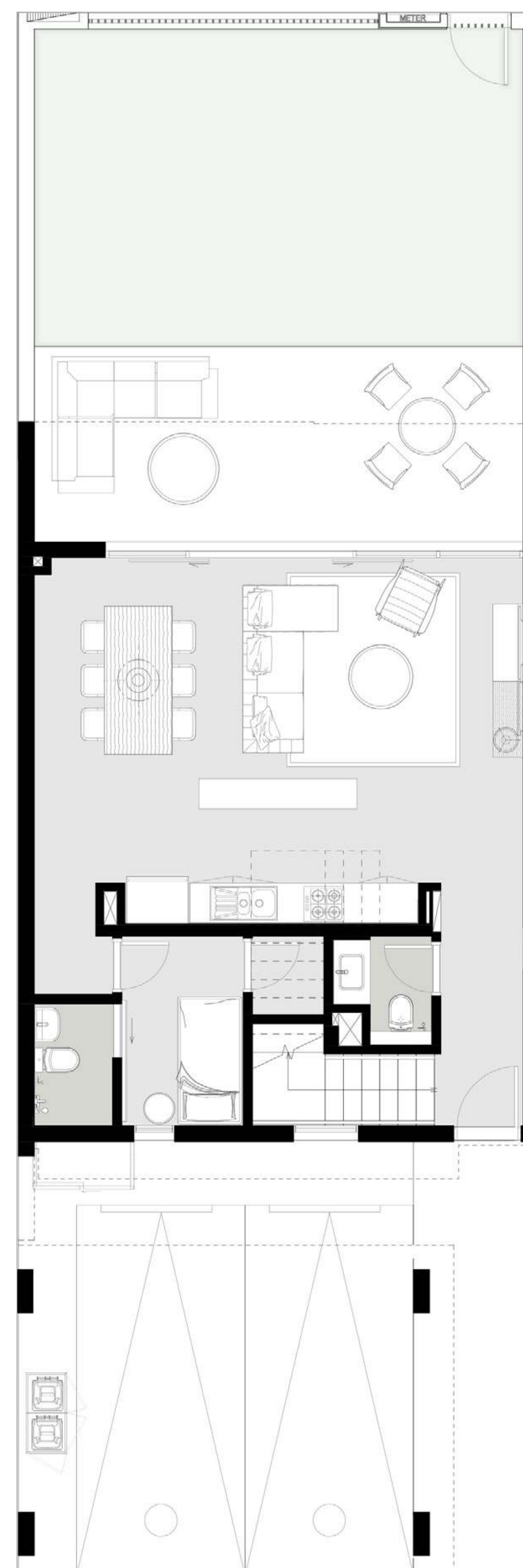
GROUND FLOOR
