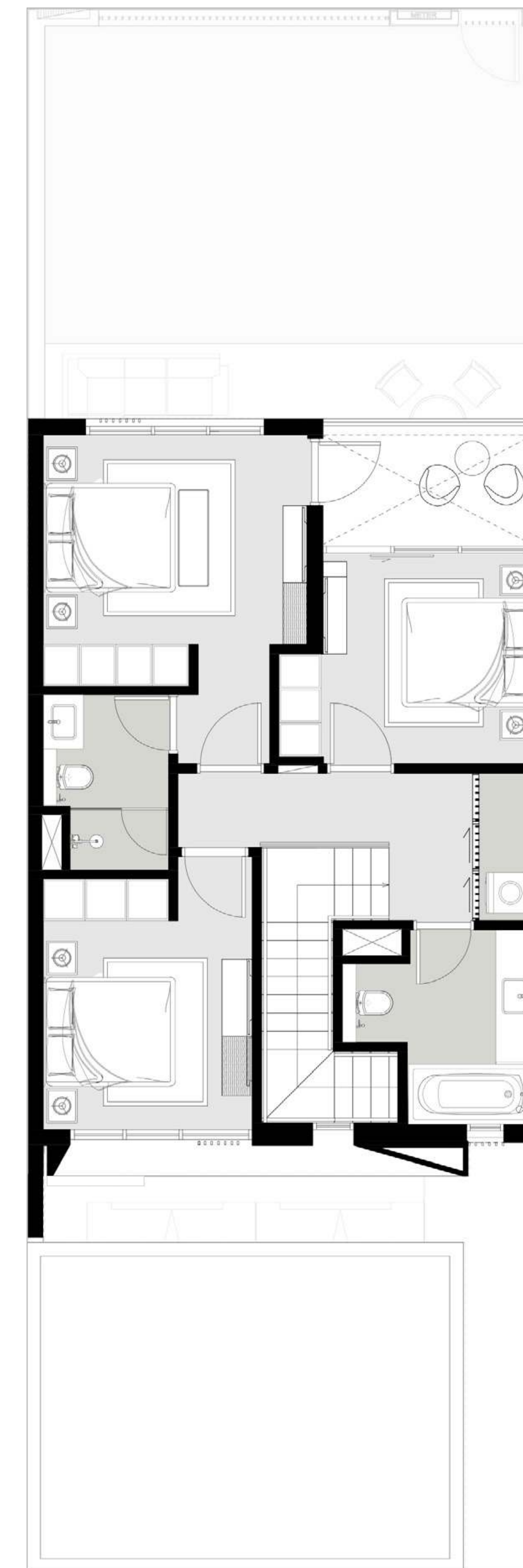
FIRST FLOOR
