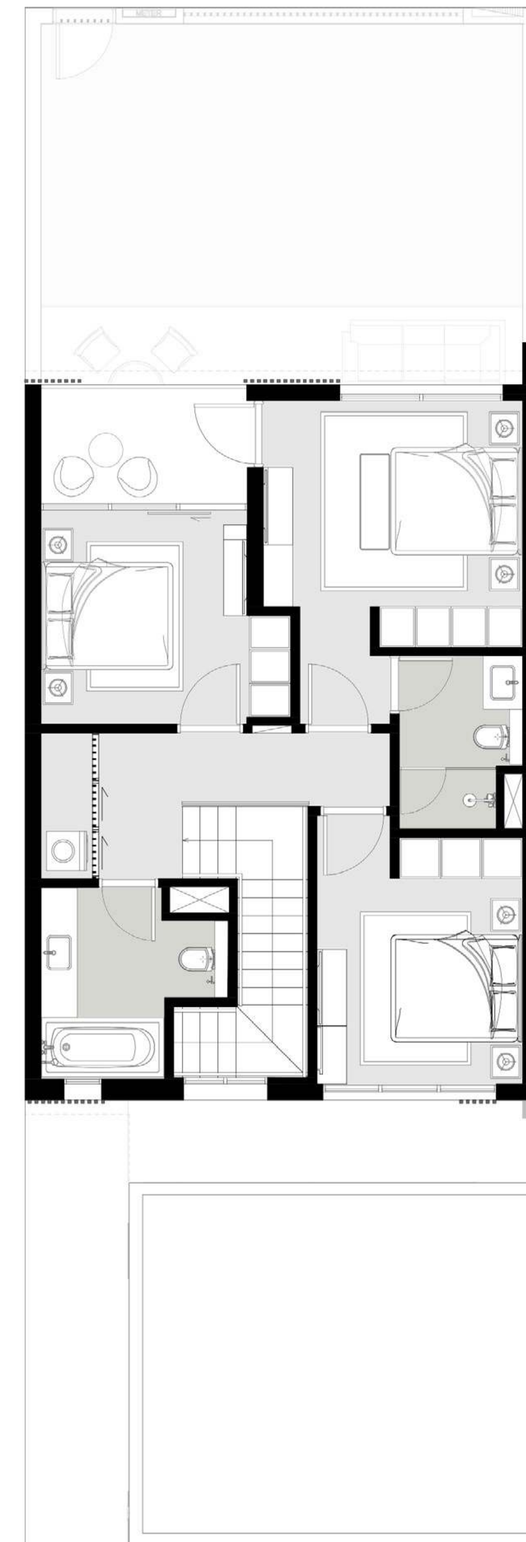
FIRST FLOOR
