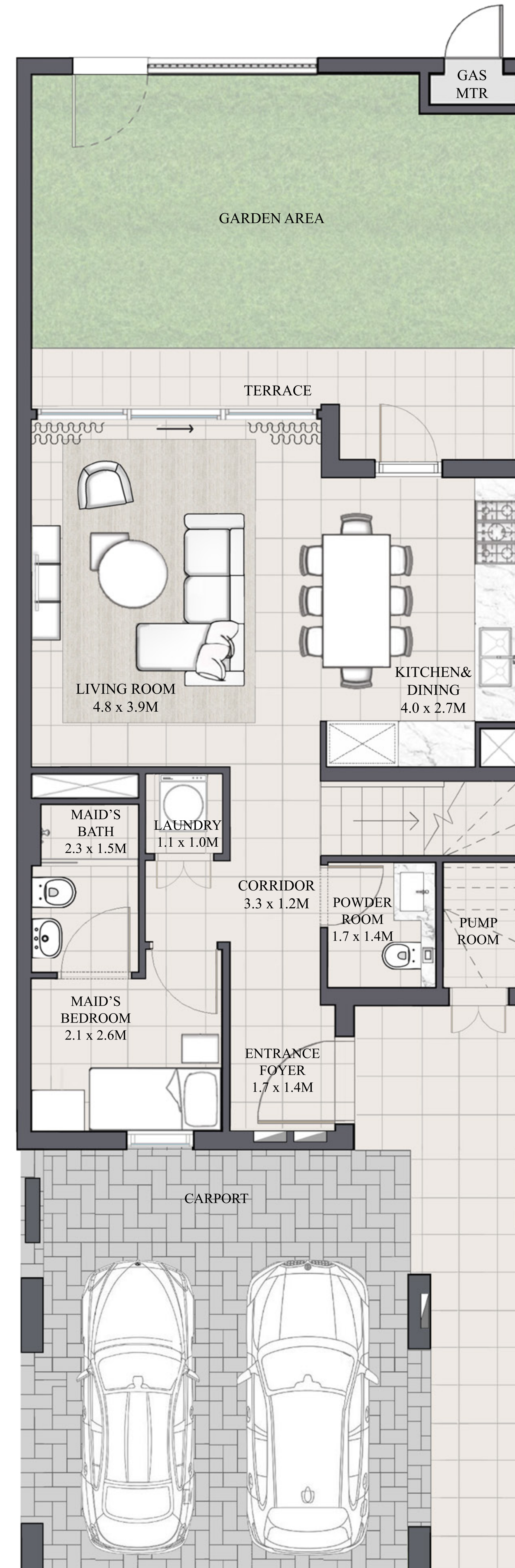
GROUND FLOOR
