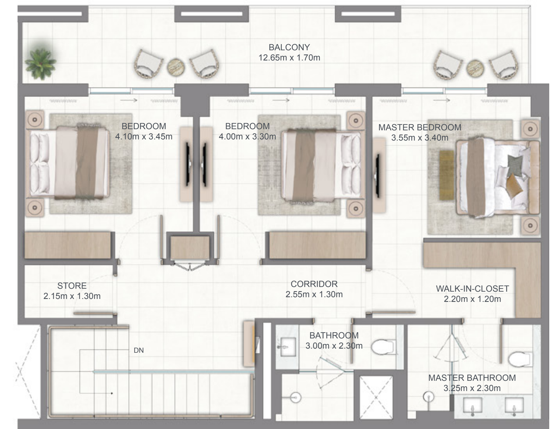
UPPER FLOOR
