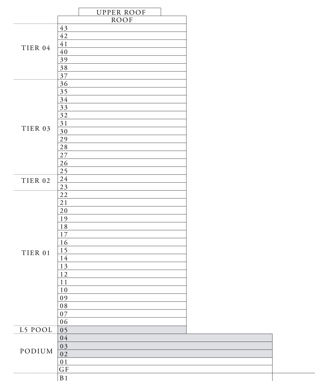
KEY SECTION
