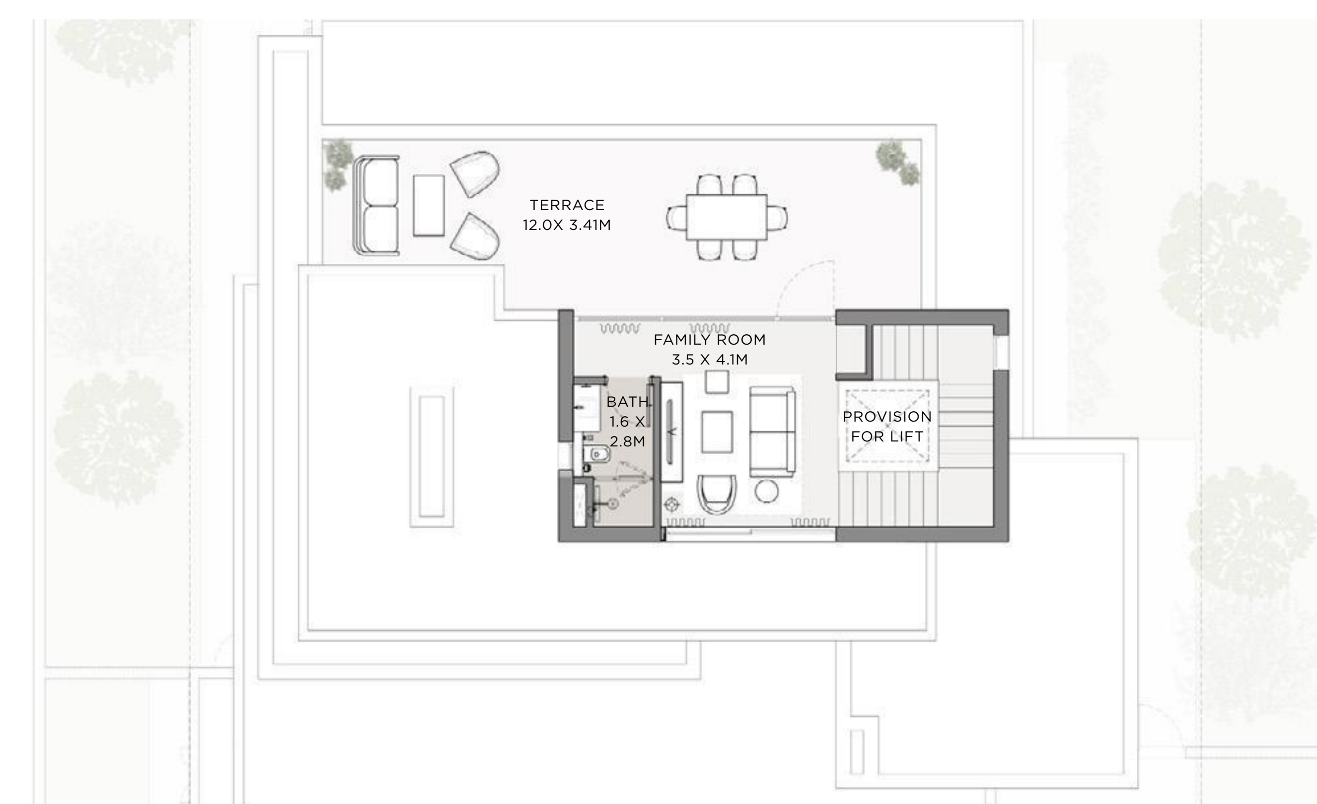
ROOF FLOOR
