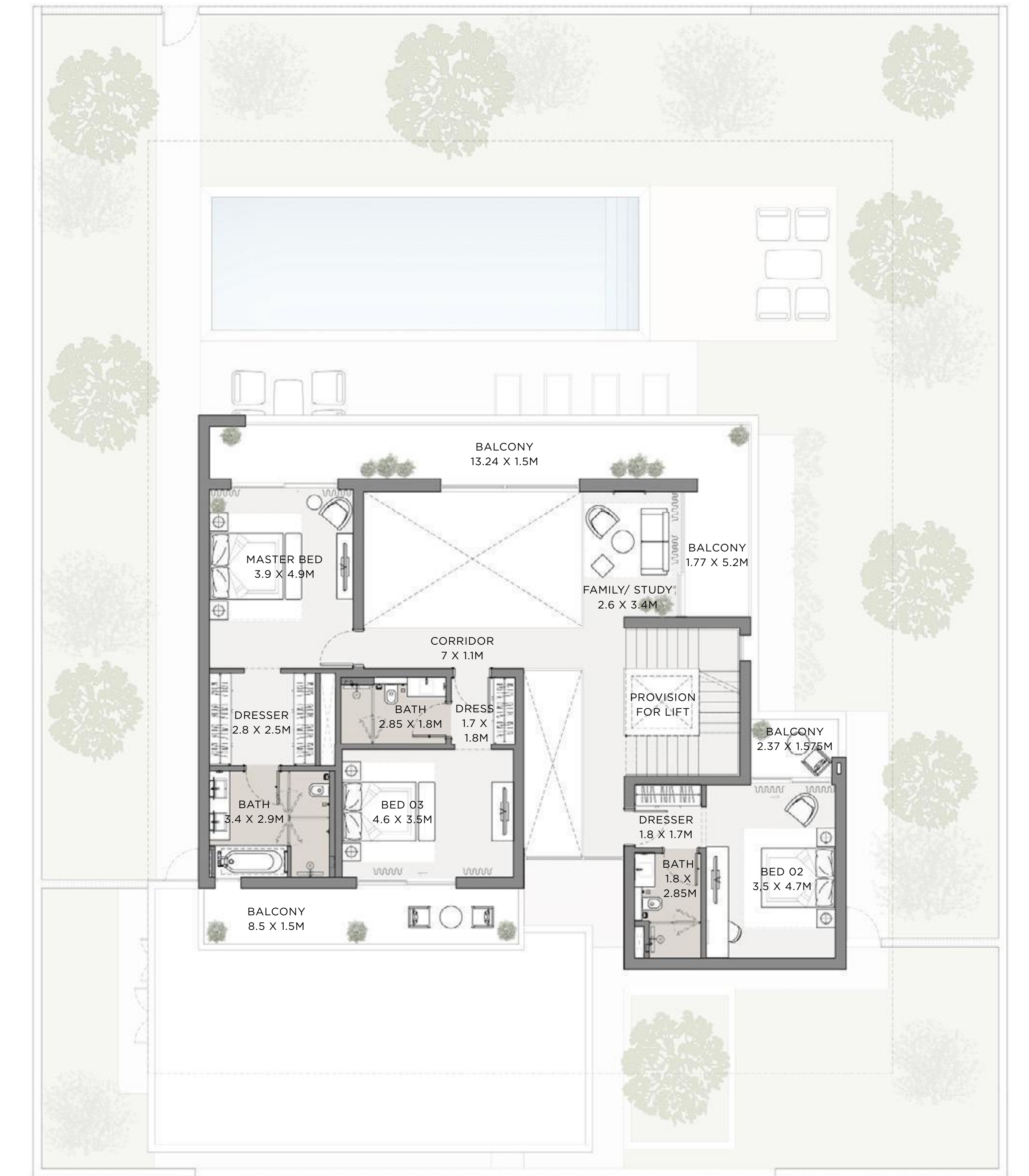
FIRST FLOOR
