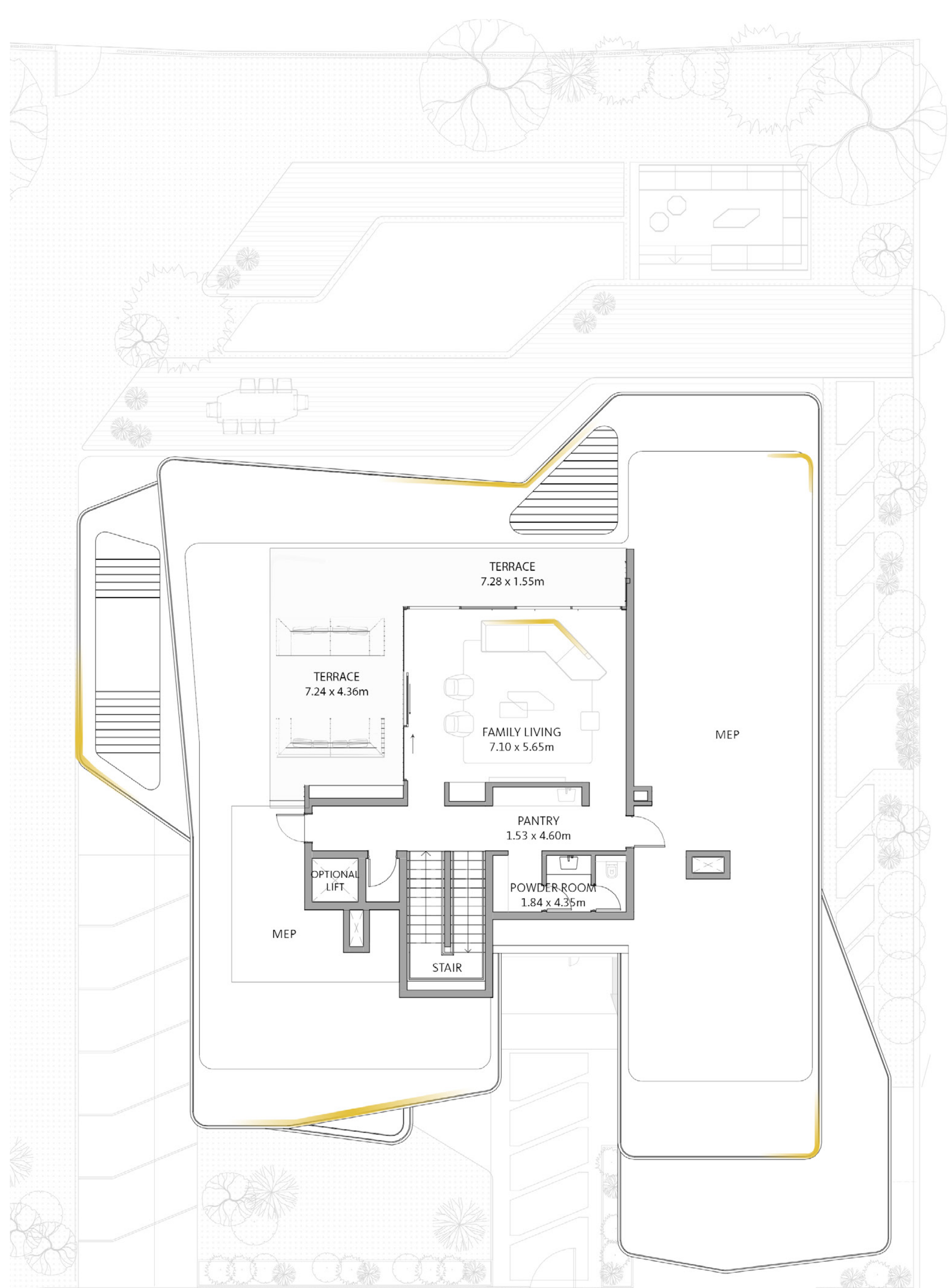
ROOF FLOOR
