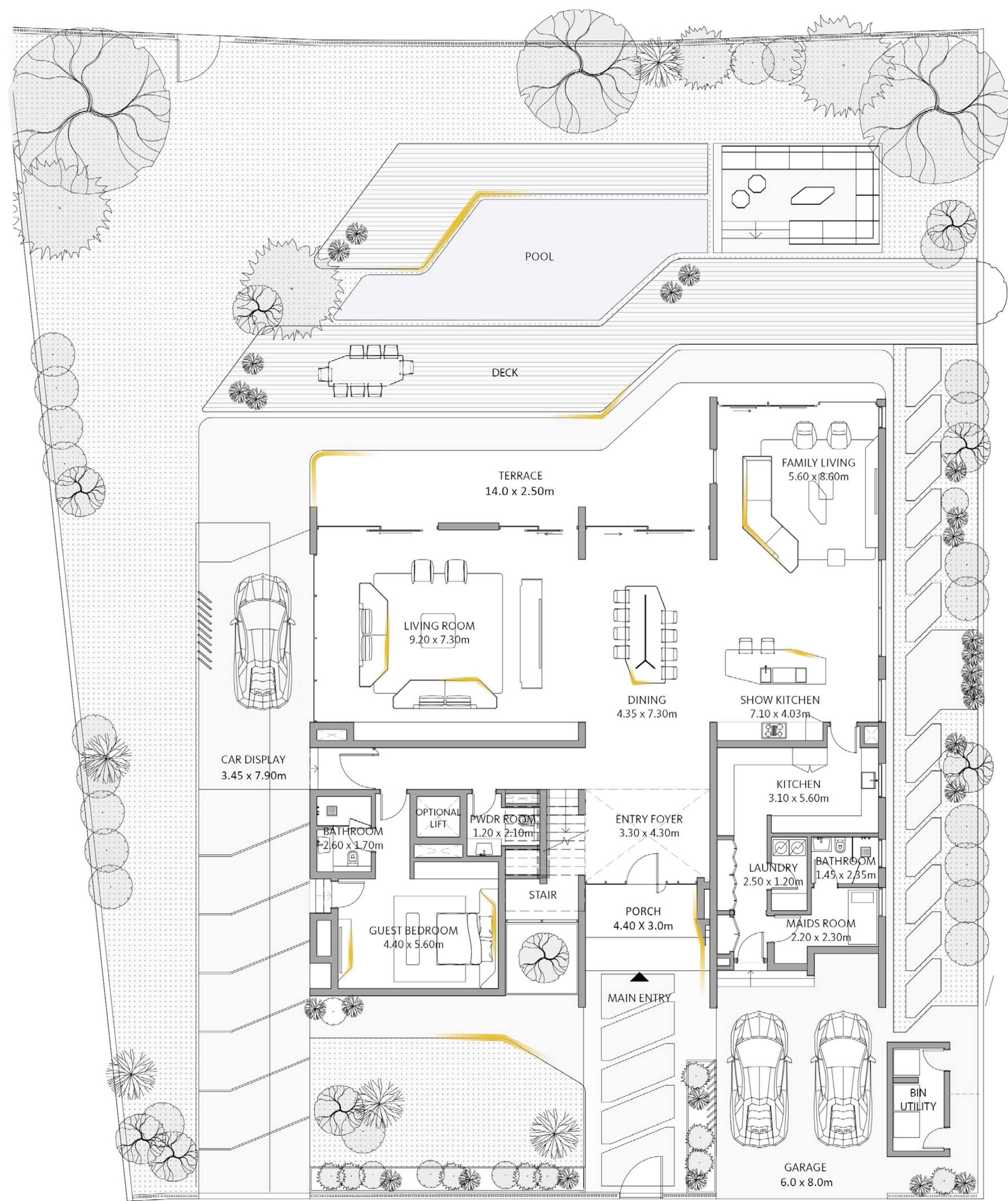
GROUND FLOOR
