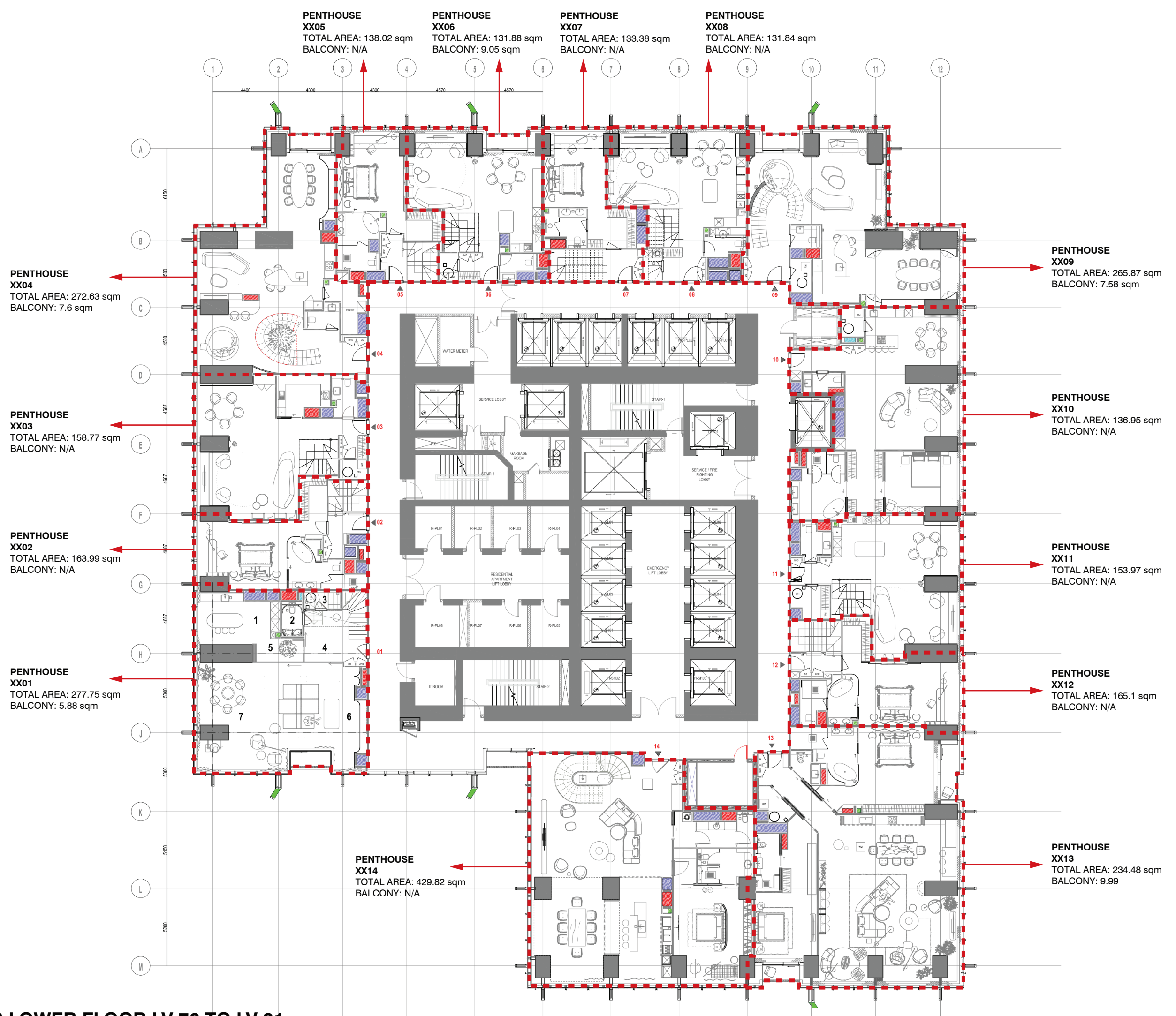
PENTHOUSE UNITS LOWER FLOOR LV 76 TO LV 91
