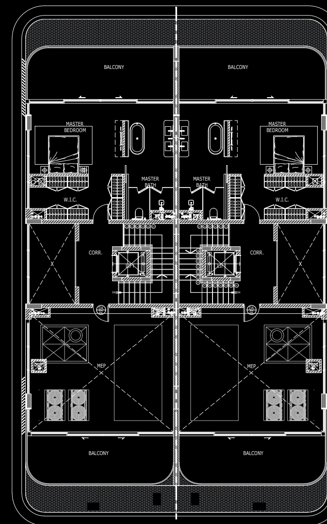
Second Floor
