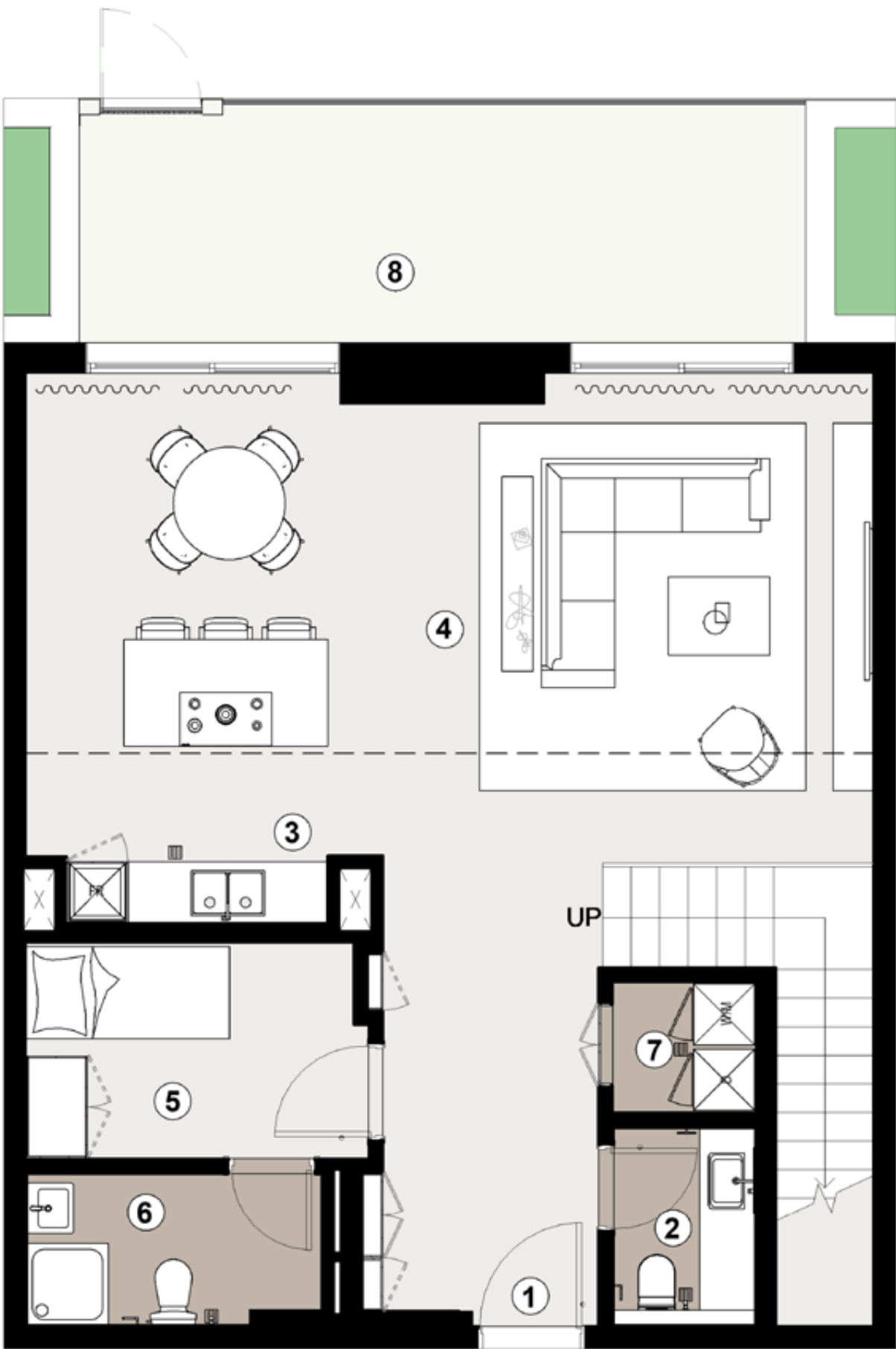
GROUND FLOOR
